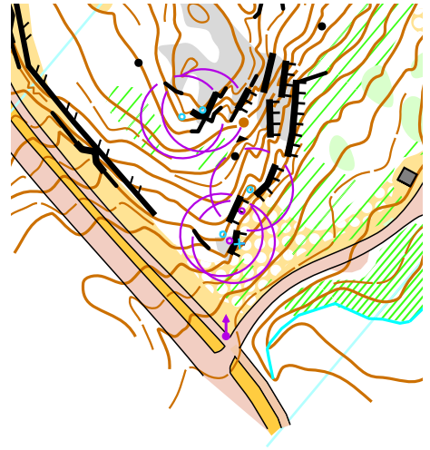
Station: 4 1:2 000
